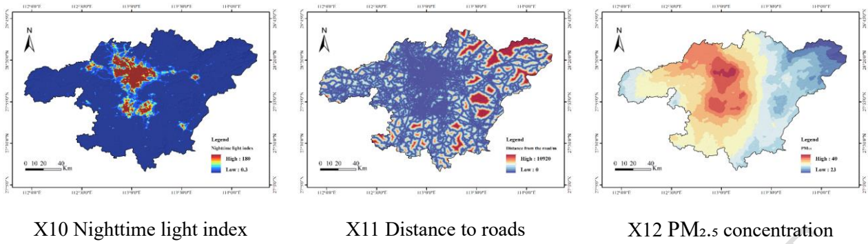
Figure 2: Spatial distribution of ecological sensitivity influencing factors in the Changsha–Zhuzhou–Xiangtan metropolitan area.
