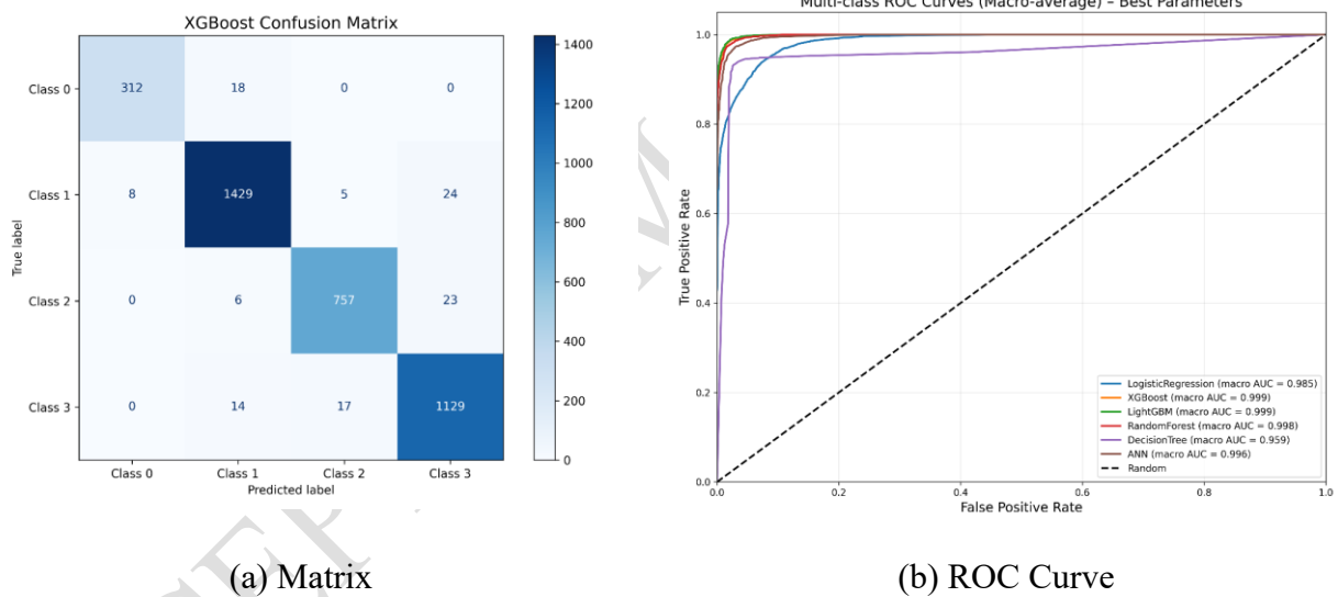
Figure 4: Model Performance Evaluation Plot
