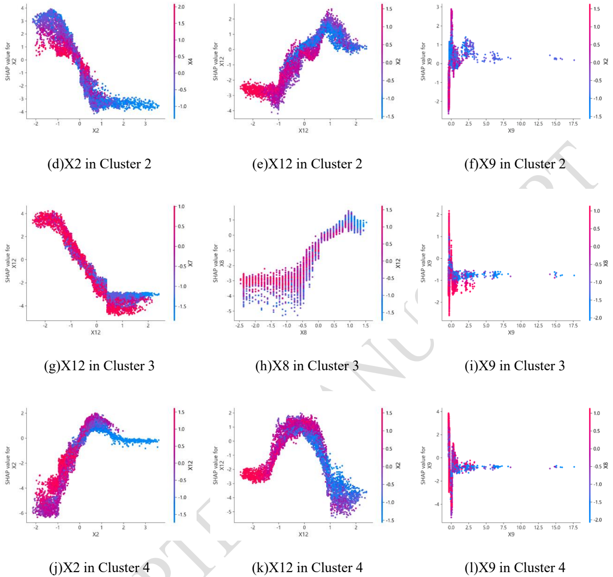
Figure 7: SHAP Feature Dependency Map of Ecological Sensitivity Factors in the Changsha-Zhuzhou-Xiangtan Metropolitan Area
