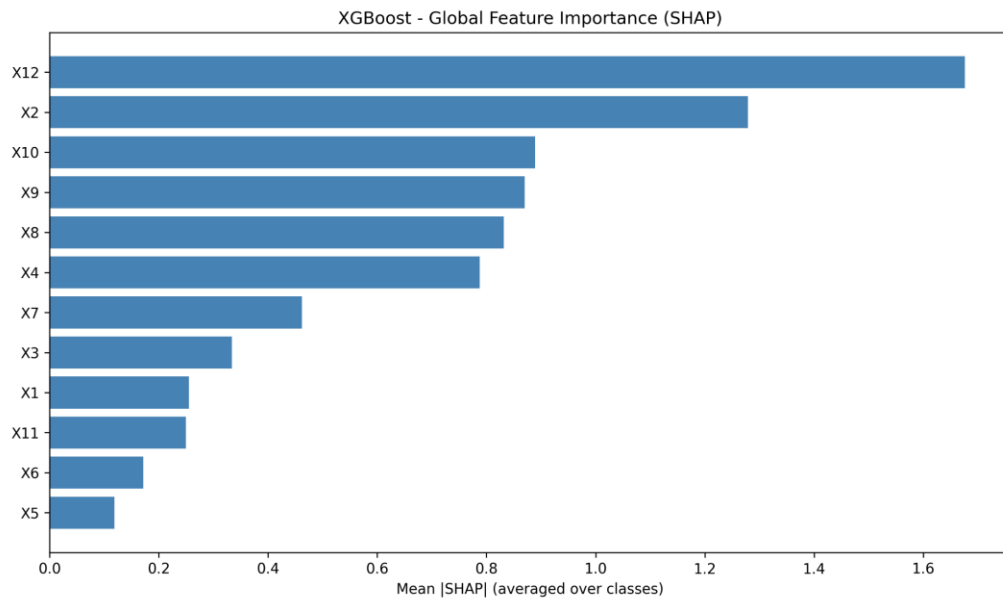
Figure 5: Importance of Ecological Sensitivity Factors in the Chang-Zhu-Tan Metropolitan Area
