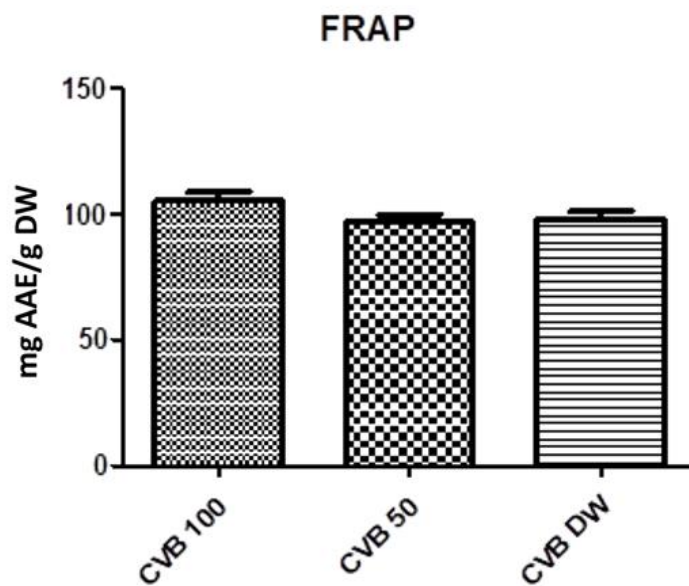
Figure 7. Ferric reducing antioxidant power (FRAP) of Cinnamomum verum bark extracts prepared using 100% methanol (CVB 100), 50% methanol (CVB 50), and distilled water (CVB DW), expressed as mg ascorbic acid equivalents per gram of dry weight (mg AAE/g DW). Values are presented as mean \pm SD of three technical measurements performed on one extract per solvent.
