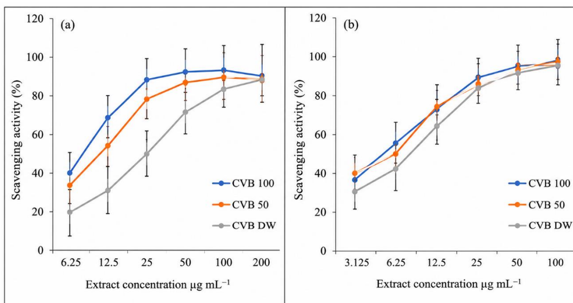
Figure 6. DPPH (a) and ABTS (b) radical scavenging activities of Cinnamomum verum bark extracts prepared using 100% methanol (CVB 100), 50% methanol (CVB 50), and distilled water (CVB DW).
