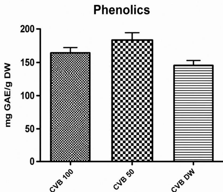
Figure 5. Total phenolic content of Cinnamomum verum bark extracts prepared using 100% methanol (CVB 100), 50% methanol (CVB 50), and distilled water (CVB DW), expressed as mg gallic acid equivalents per gram of dry weight (mg GAE/g DW). Values are presented as mean \pm SD of three technical measurements performed on one extract per solvent.
