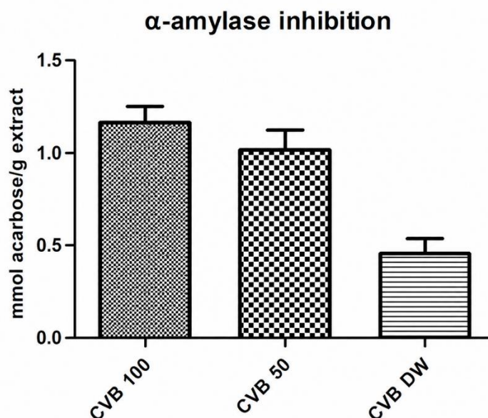
Figure 1. \alpha -Amylase inhibitory activity of Cinnamomum verum bark extracts prepared using 100% methanol (CVB 100), 50% methanol (CVB 50), and distilled water (CVB DW), expressed as mmol acarbose equivalents per gram of extract. Values are presented as mean \pm SD of three technical measurements performed on one extract per solvent.
