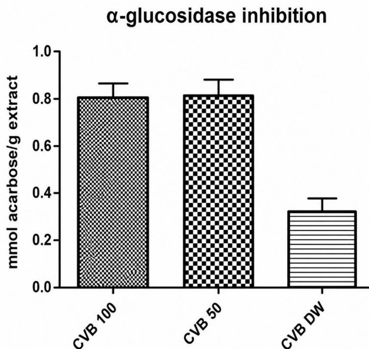
Figure 2. \alpha -glucosidase inhibitory activity of Cinnamomum verum bark extracts prepared using 100% methanol (CVB 100), 50% methanol (CVB 50), and distilled water (CVB DW), expressed as mmol acarbose equivalents per gram of extract. Values are presented as mean \pm SD of three technical measurements performed on one extract per solvent.
