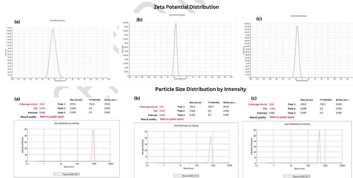
Figure 9. Zeta potential and Particle size distribution (intensity-based) of (a) \text{g-C}_3\text{N}_4 , (b) \text{Mo}_{0.5}\text{Mn}_{0.5}\text{Fe}_2\text{O}_4 nanoparticles, (c) \text{Mo}_{0.5}\text{Mn}_{0.5}\text{Fe}_2\text{O}_4/\text{g-C}_3\text{N}_4 nanocomposites
