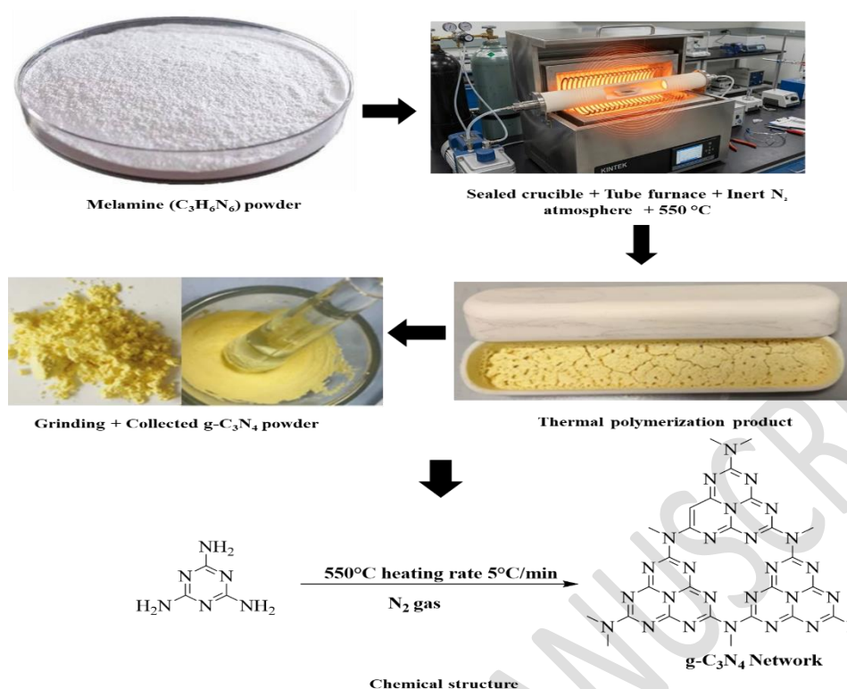
Figure 1. Synthesis of g-C_3N_4
