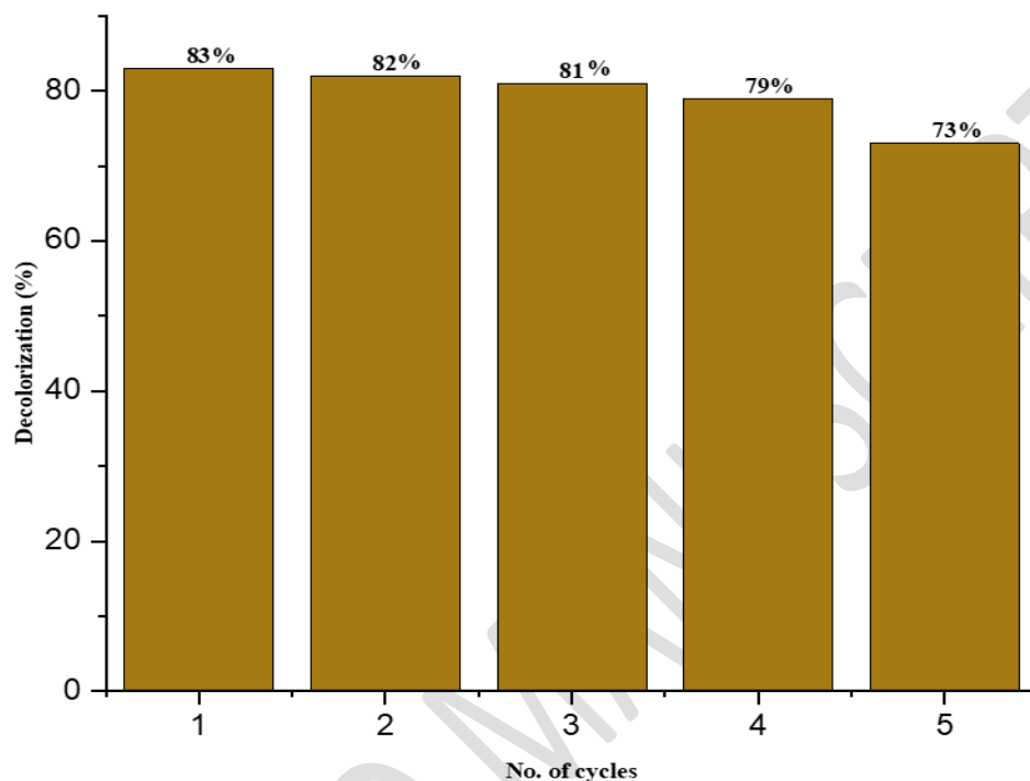
Figure 16. Catalyst reusability
