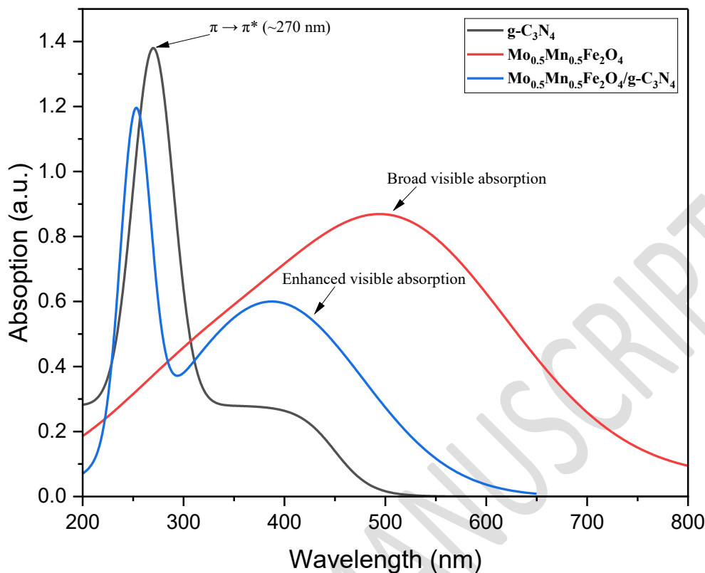
Figure 4. Comparison UV-visible graph of (a) pristine g-C 3 N 4 , (b) Mo 0.5 Mn 0.5 Fe 2 O 4 nanoparticles, (c) Mo 0.5 Mn 0.5 Fe 2 O 4 /g-C 3 N 4 nanocomposites.
