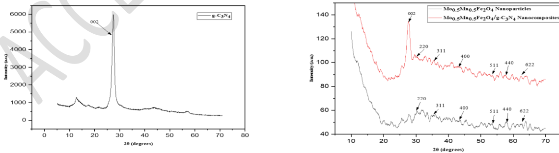
Figure 5. XRD images of (a) pristine \text{g-C}_3\text{N}_4 (b) \text{Mo}_{0.5}\text{Mn}_{0.5}\text{Fe}_2\text{O}_4 nanoparticles, \text{Mo}_{0.5}\text{Mn}_{0.5}\text{Fe}_2\text{O}_4/\text{g-C}_3\text{N}_4 nanocomposites,
