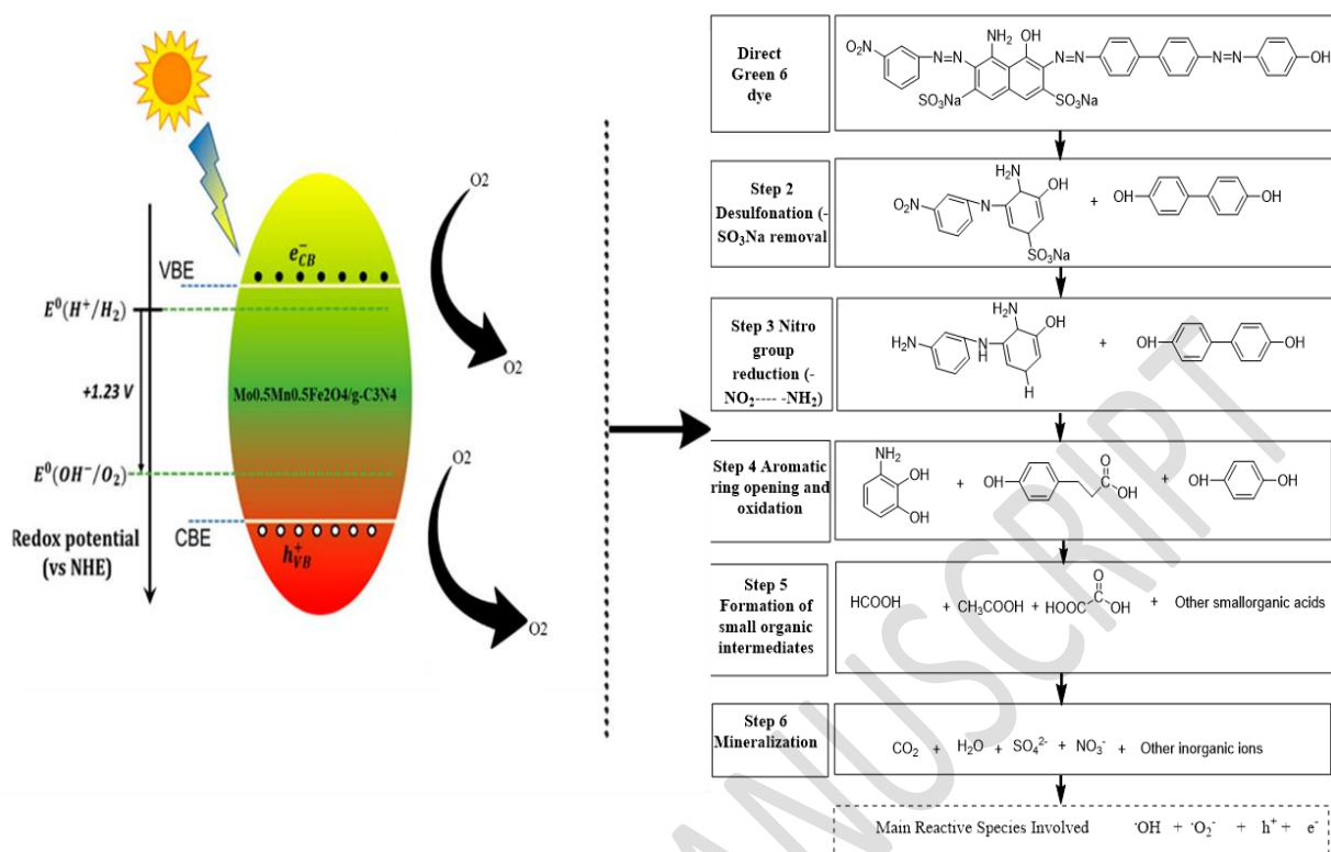
Figure 18. Proposed mechanism of degradation of Direct Green 6 dye (DG6) over \text{Mo}_{0.5}\text{Mn}_{0.5}\text{Fe}_2\text{O}_4/\text{g-C}_3\text{N}_4 nanocomposite under visible-light irradiation
