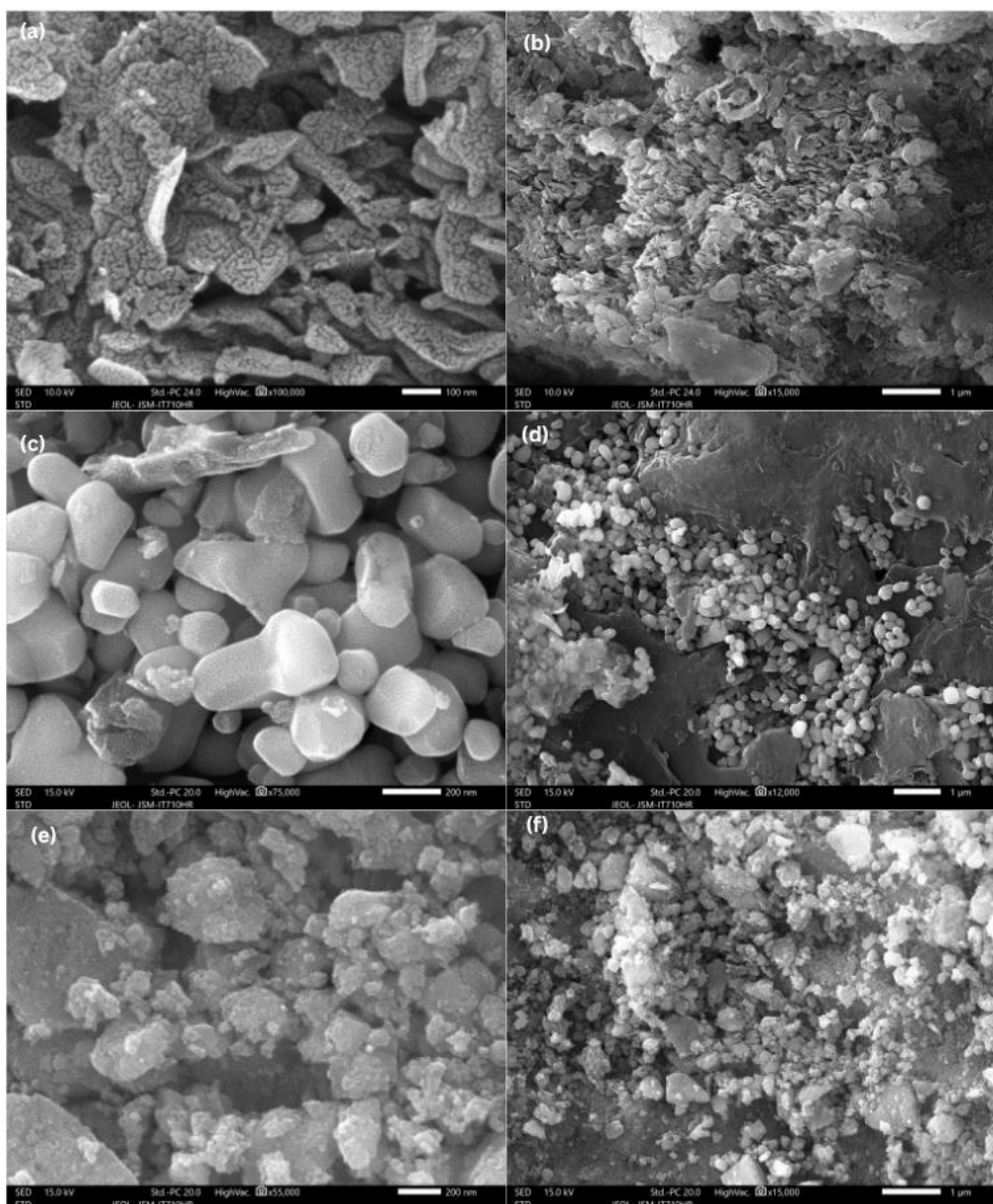
Figure 6. SEM analysis of (a) and (b) g-C 3 N 4 , (c) and (d) Mo 0.5 Mn 0.5 Fe 2 O 4 nanoparticles, (e) and (f) Mo 0.5 Mn 0.5 Fe 2 O 4 /g-C 3 N 4 nanocomposites
