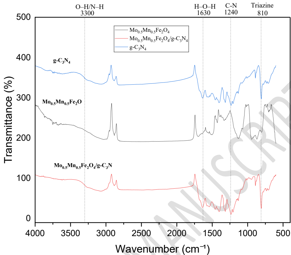
Figure 8. Comparison of FTIR spectrum of pristine \text{g-C}_3\text{N}_4 , \text{Mo}_{0.5}\text{Mn}_{0.5}\text{Fe}_2\text{O}_4 nanoparticles, and their \text{Mo}_{0.5}\text{Mn}_{0.5}\text{Fe}_2\text{O}_4/\text{g-C}_3\text{N}_4 nanocomposites
