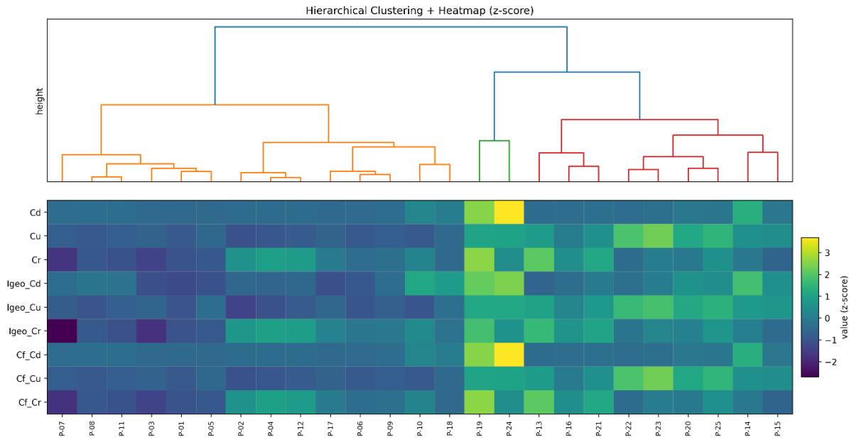
Figure 11. Hierarchical Clustering and Z-Score Heatmap of Heavy Metals (Cd, Cu, Cr) and Associated Contamination Indices (Igeo and CF) Across Sampling Sites
