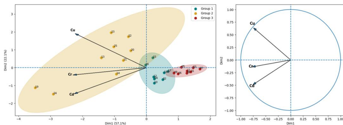
Figure 9. Principal component analysis (PCA) of heavy metals in urban soils showing (a) the biplot of sampling sites grouped into three clusters and (b) the correlation circle of Cd, Cu, and Cr.
