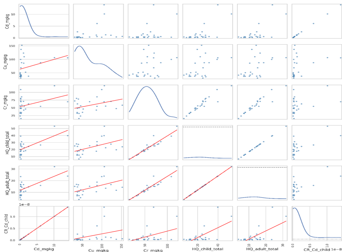
Figure 13. Pairwise relationships between heavy metal concentrations (Cd, Cu, Cr) and human health risk indicators (HQ and CR) for different age groups in urban soils.
