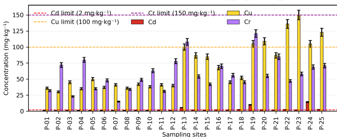
Figure 4. Concentrations of Cd, Cu, and Cr in soil samples collected from the Annaba City region.
