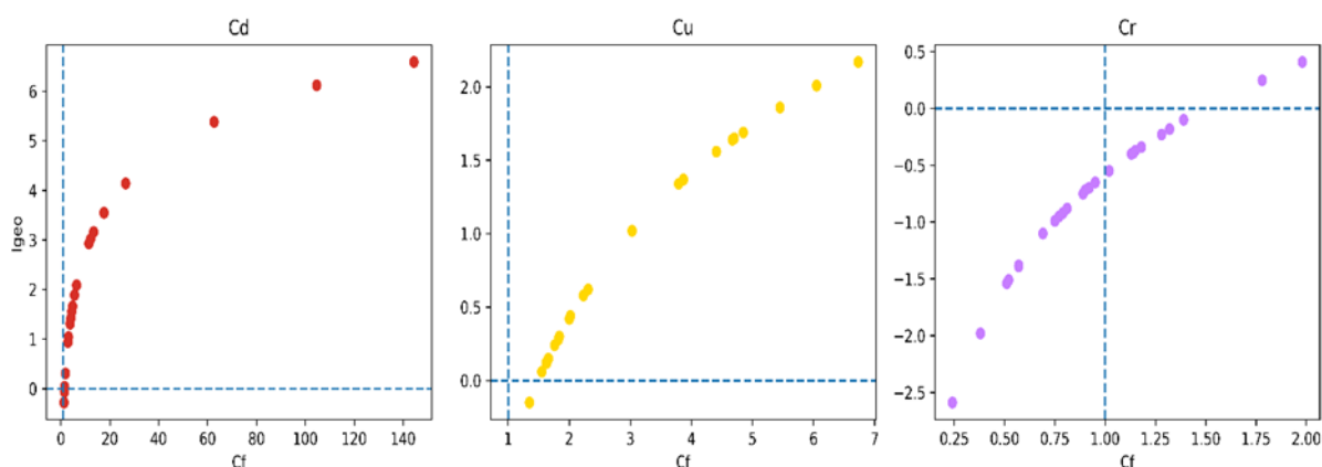
Figure 7. Relationship between the geo-accumulation index (Igeo) and contamination factor (CF) for Cd, Cu, and Cr in soils from the Annaba City region.
