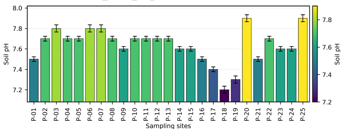
Figure 3. Spatial variation of soil pH across sampling sites in the Annaba City region.
