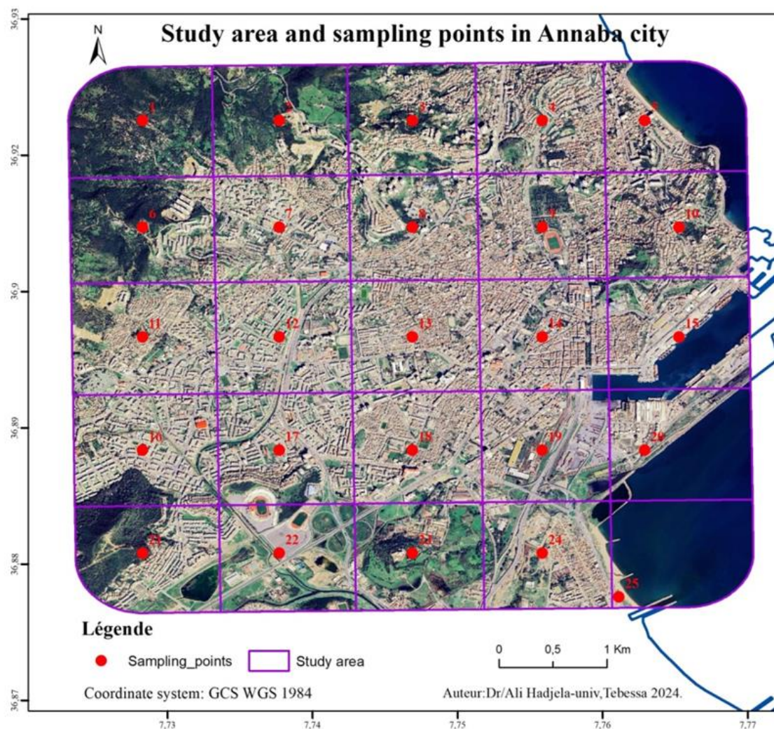
Figure 2. Sampling points and geographic coordinates in decimal degrees of 25 soil samples from the Annaba City region.
