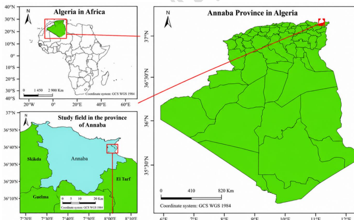
Figure 1. Geographic location of the study area soil samples in Annaba City (top map).
