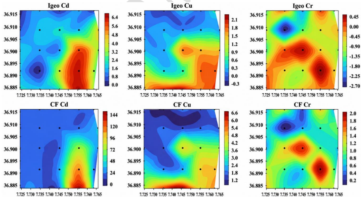
Figure 6. Spatial distribution of geo-accumulation index ( Igeo ) and contamination factor ( CF ) for Cd, Cu, and Cr in urban soils from the Annaba City region..
