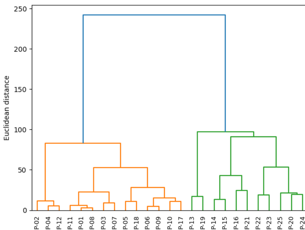
Figure 10. Hierarchical cluster analysis (HCA) dendrogram of urban soil samples based on Cd, Cu, and Cr concentrations using Ward's linkage method and Euclidean distance.
