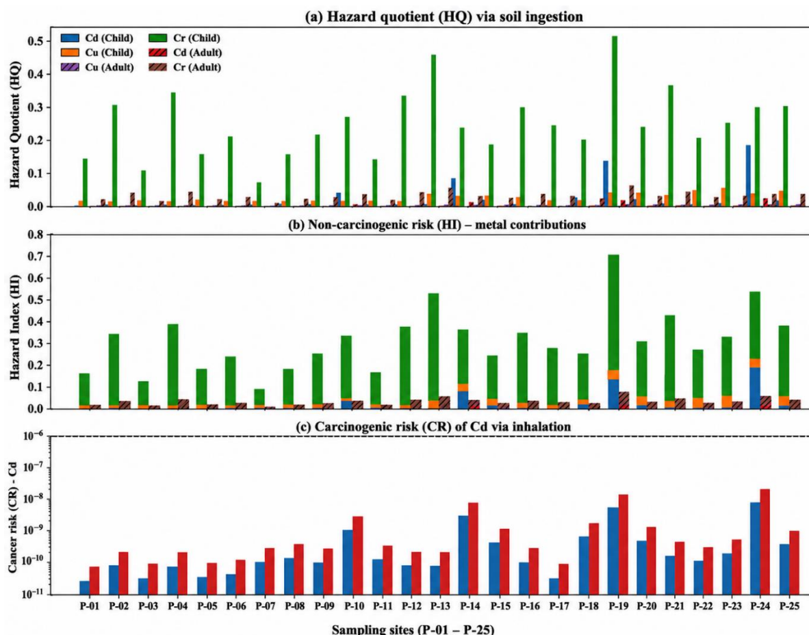
Figure 8. presents the integrated human health risk assessment of heavy metals in urban soils using hazard quotient (HQ), hazard index (HI), and carcinogenic risk (CR) indicators for children and adults
