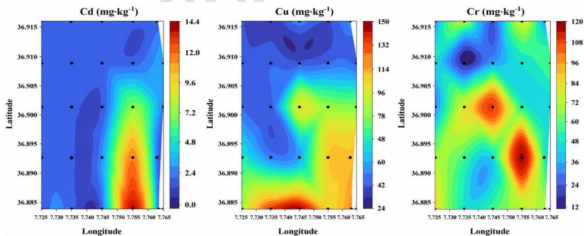
Figure 5. Spatial distribution of Cd, Cu and Cr concentrations in urban soils from the Annaba City region.
