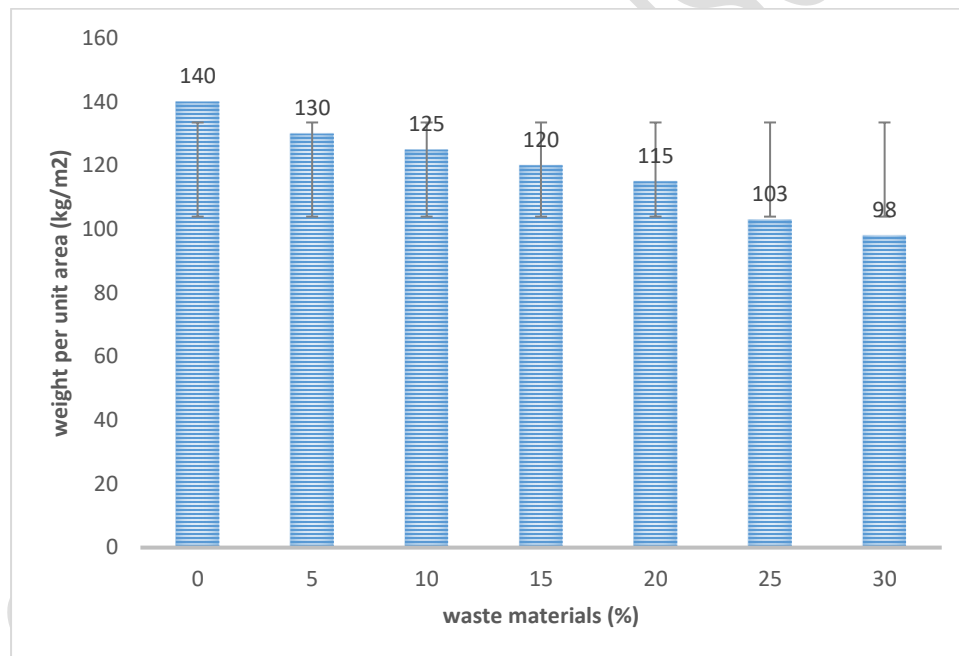
Figure. 7 Mass per surface area of brick specimens incorporating waste materials and sugarcane bagasse ash
