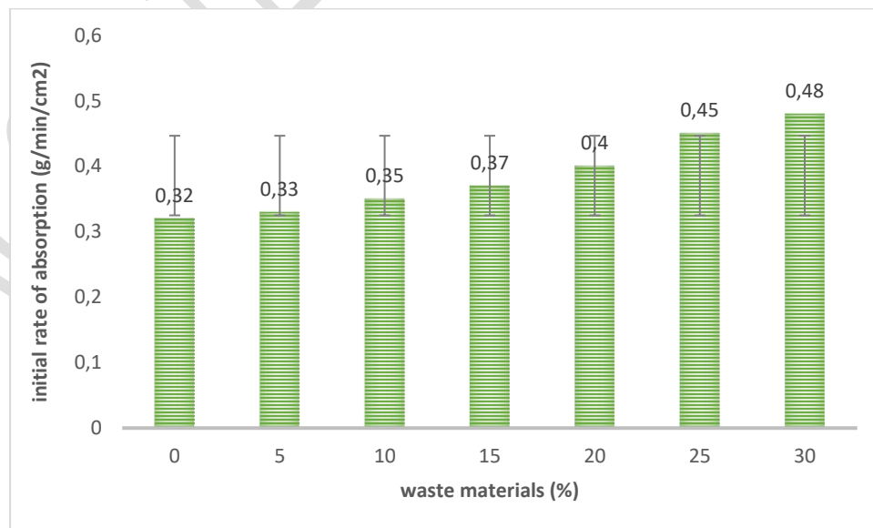
Figure 9. Initial moisture absorption behavior of bricks containing waste
