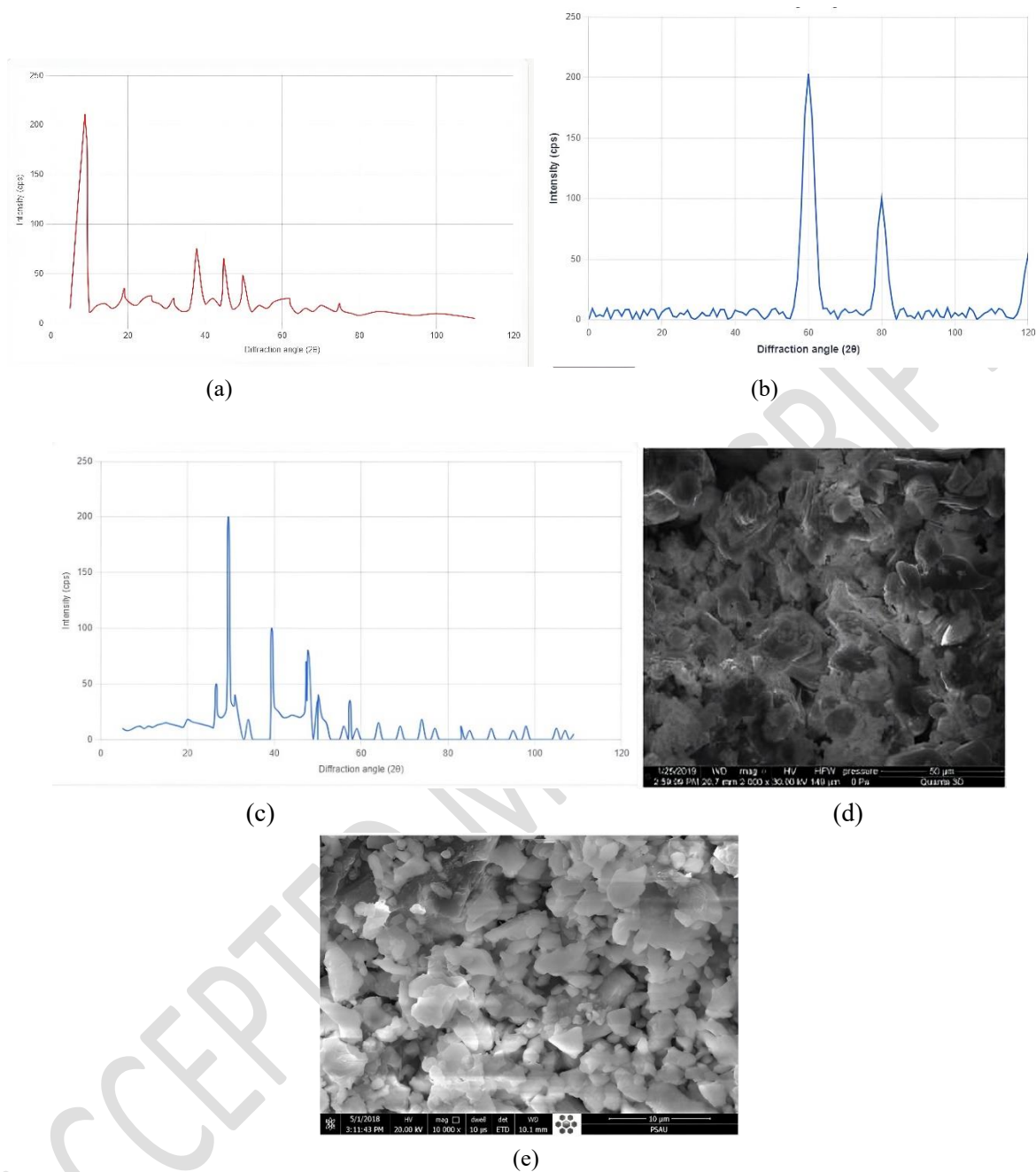
Figure 5 XRD and SEM profiles of the materials (a) Clay, (b, e) sugarcane bagasse, (c, d) Marble waste powder
