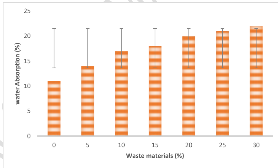
Figure 8 Water absorption characteristics of bricks made with WMP and SBA
