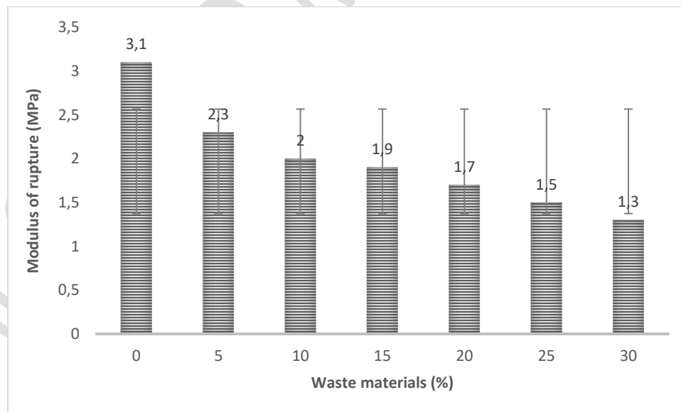
Figure 12: Modulus of rupture of brick specimens
