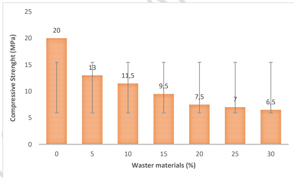
Figure 11: Compressive Strength of Brick Specimens
