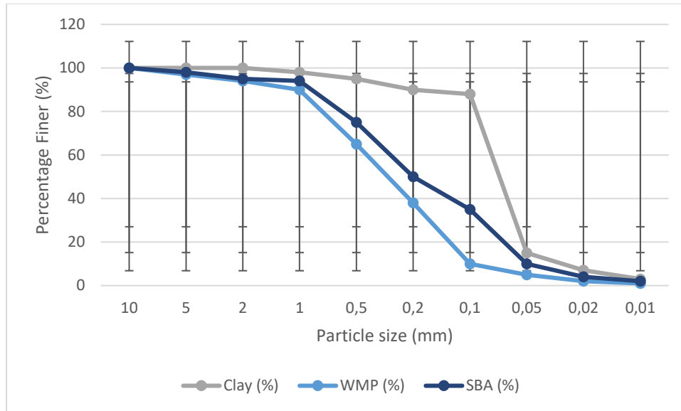
Figure. 6 Particle Distribution Curve for Clay, WMP, SBA
