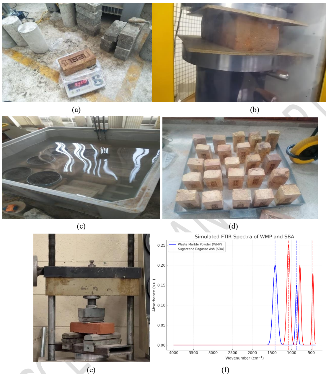
Figure 4. (a) Dry weight of Brick, (b) Compressive Strength, (c) water absorption, (d) Specimens Placed in water for efflorescence, (e) Flexural Strength, (f) FTIR analysis
