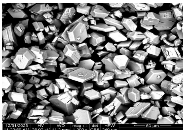
Figure 3. SEM images of POM-Fe.
