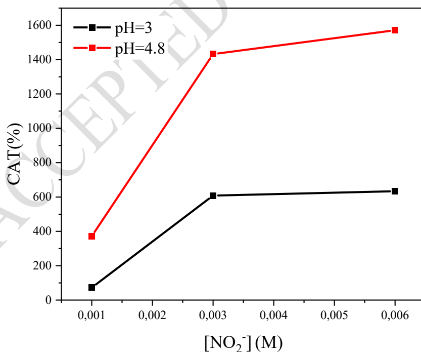
Figure 15. Variation of catalytic efficiency (%) as a function of nitrite concentration (mean \pm SD, n = 3).
