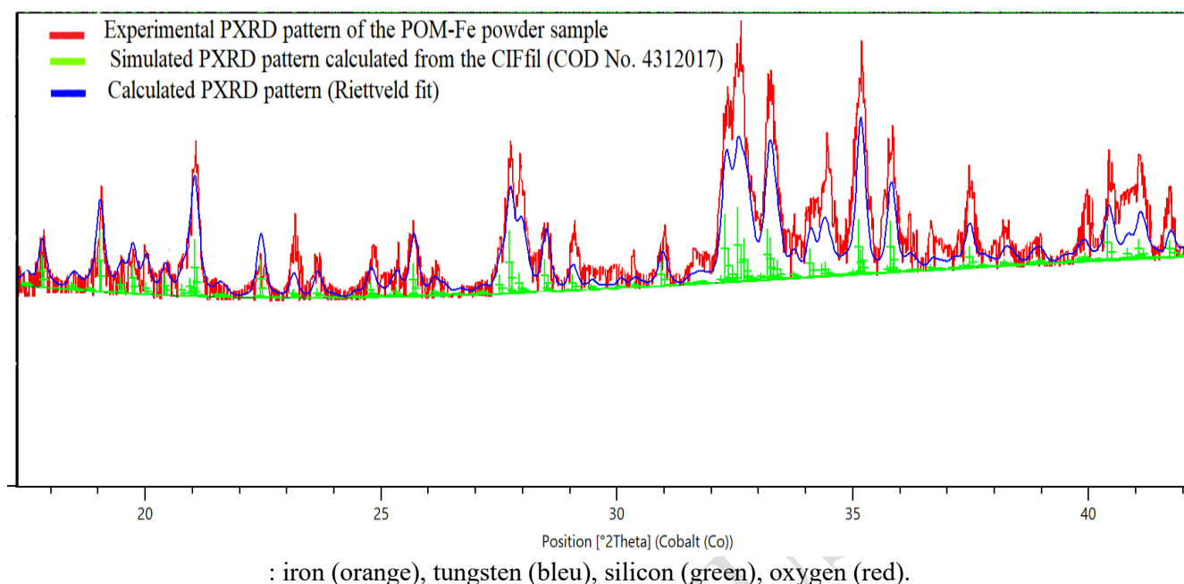
Figure 6. Experimental powder X-ray diffraction (PXRD) pattern of the POM–Fe powder compared with the simulated pattern calculated from the CIF file (COD No. 4312017) and the refined pattern obtained from Rietveld analysis.
