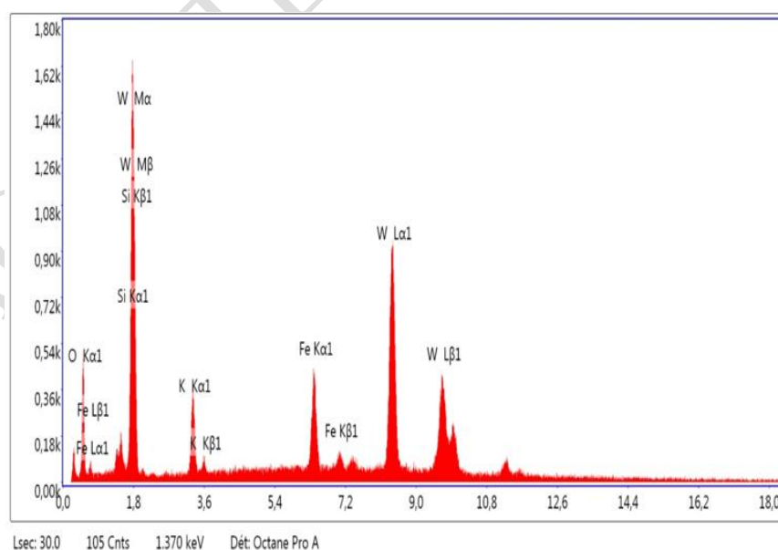
Figure 4. EDX spectrum of POM-Fe.
