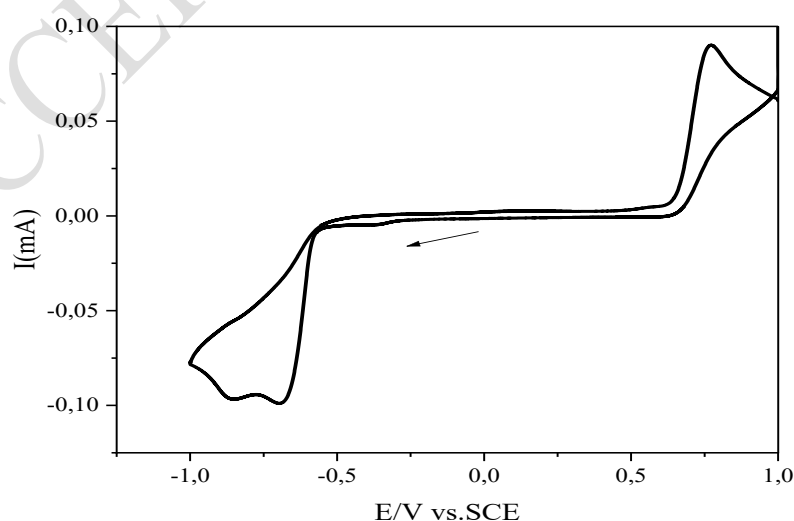
Figure 14. Cyclic voltammetry after two-step electrolysis ( -400 and -900 mV vs. SCE), highlighting the \text{Fe}^{2+} \rightarrow \text{Fe}^{3+} anodic oxidation wave at +0.70 V.
