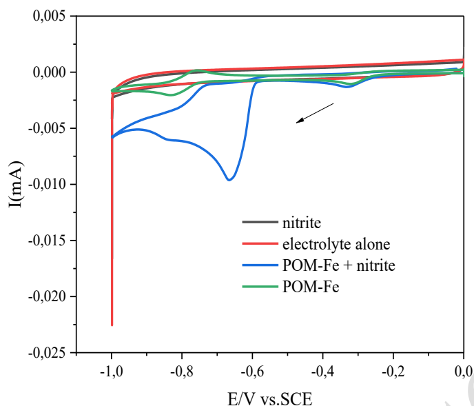
Figure 12. Comparative cyclic voltammetry of nitrite, electrolyte alone, POM-Fe, and POM-Fe with nitrite.
