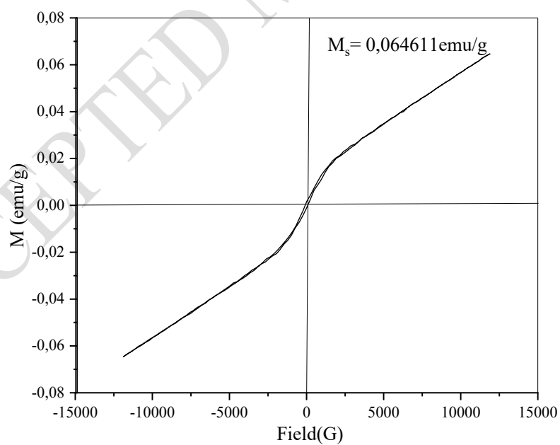
Figure 8. VSM curve of POM-Fe.
