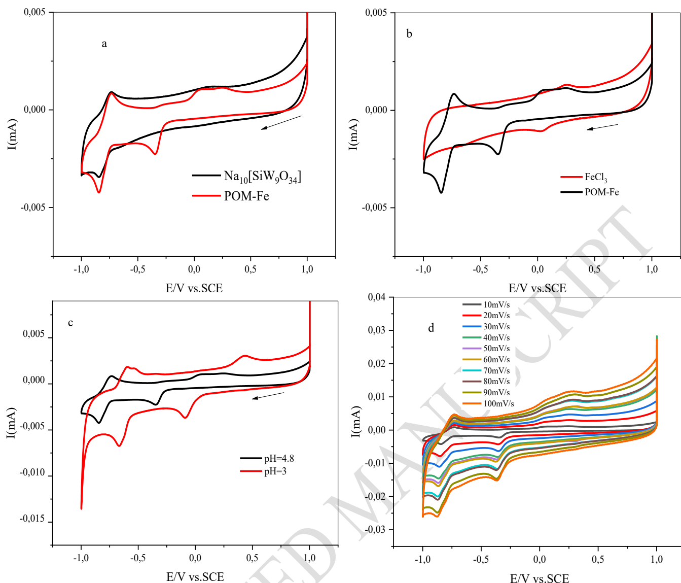
Figure 9. (a) CV of POM-Fe and \text{Na}_{10}[\text{SiW}_9\text{O}_{34}] . (b) CV of POM-Fe and \text{FeCl}_3 . (c) Comparison of CV of POM-Fe at pH 3 and 4.8. C_{(\text{POM-fe})} = 1 \times 10^{-4} \text{M} , C_{\text{Na}_{10}[\text{SiW}_9\text{O}_{34}]} = 1 \times 10^{-4} \text{M} and C_{(\text{FeCl}_3)} = 1 \times 10^{-4} \text{M} , scan rate 10 \text{ mV.s}^{-1} (d) CV of POM-Fe recorded at scan rates varying from 10 to 100 \text{ mV.s}^{-1} .
