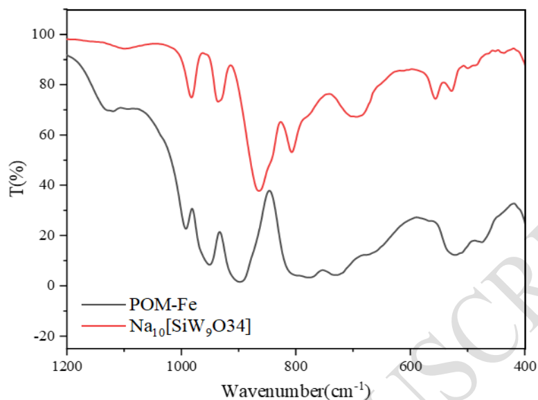
Figure 1. IR spectra of the polyoxometallates \alpha -Na 10 [SiW 9 O 34 ] and POM-Fe.
