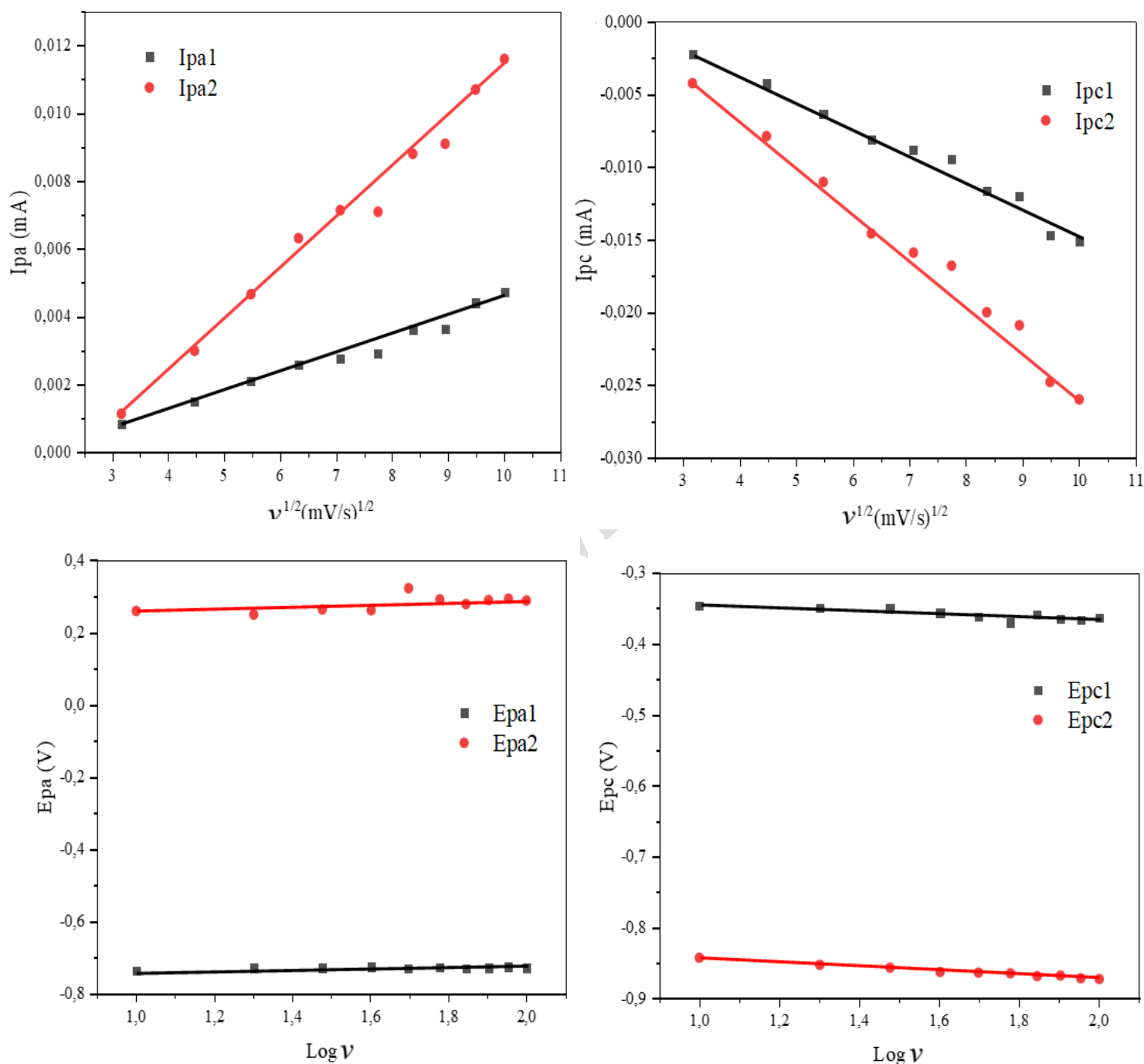
Figure 10. Relationship of I_{pc} and I_{pa} vs square root of scan rate ( v^{1/2} ) and \log v at 25°C.
