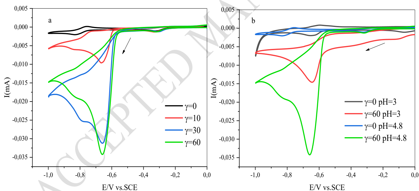
Figure 11. (a): Nitrite Electroreduction in the presence of 1 \times 10^{-4} M POM-Fe in acetate buffer at pH 4.8. (b): Comparison of nitrite Electroreduction at pH 4.8 and pH 3 medium. The scan rate v = 2 \text{ mV} \cdot \text{s}^{-1} .
