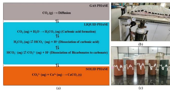
Figure 2. (a) Carbonation reaction process; (b) Carbonation curing unit; (c) Ambient cured samples.
