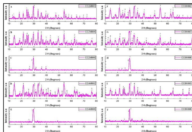
Figure 5. XRD patterns of carbonation cured samples (1:Alite, 2:Calcite, 3:Hematite, 4:N-A-S-H, 5:Quartz, 6:Thermonatrite, 7:C-A-S-H, 8:Titanium oxide)
