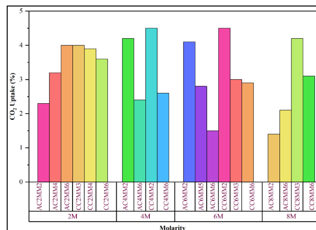
Figure 10. Comparison of \text{CO}_2 Uptake among various mix composition with molarity
