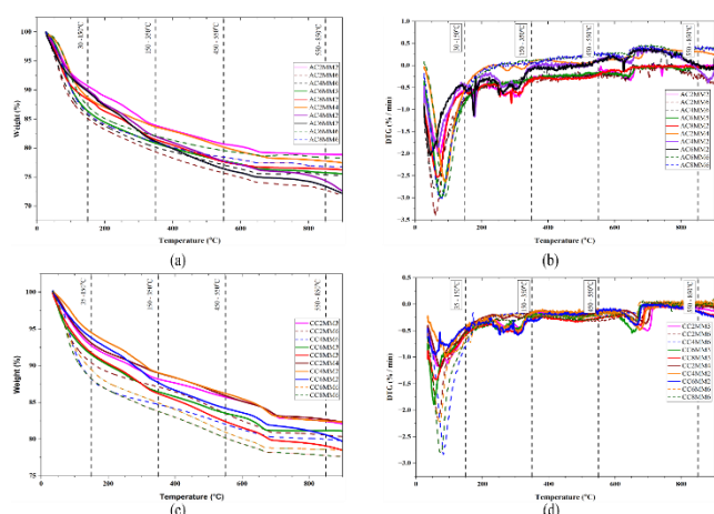
Figure 9. (a) TG Curve of ambient cured sample, (b) DTG curve of ambient cured samples, (c) TG curve of carbonation cured samples and (d) DTG curve of carbonation cured samples
