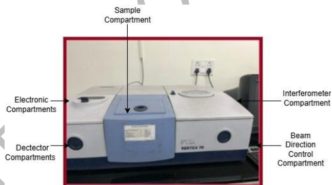
Figure 4. General FTIR Spectrometer view.
