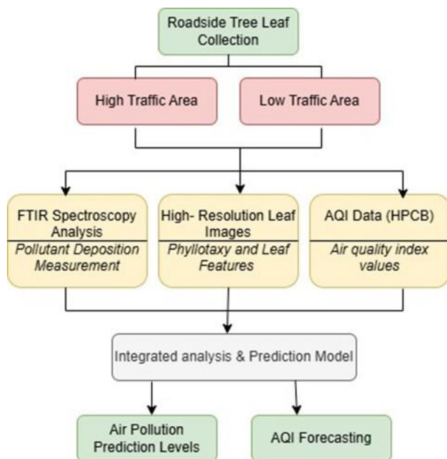
Figure 2. Proposed Model Phyllo-ViT (Phyllotaxy Vision Transform Model for Air Pollution Prediction using Machine learning) theoretical framework
