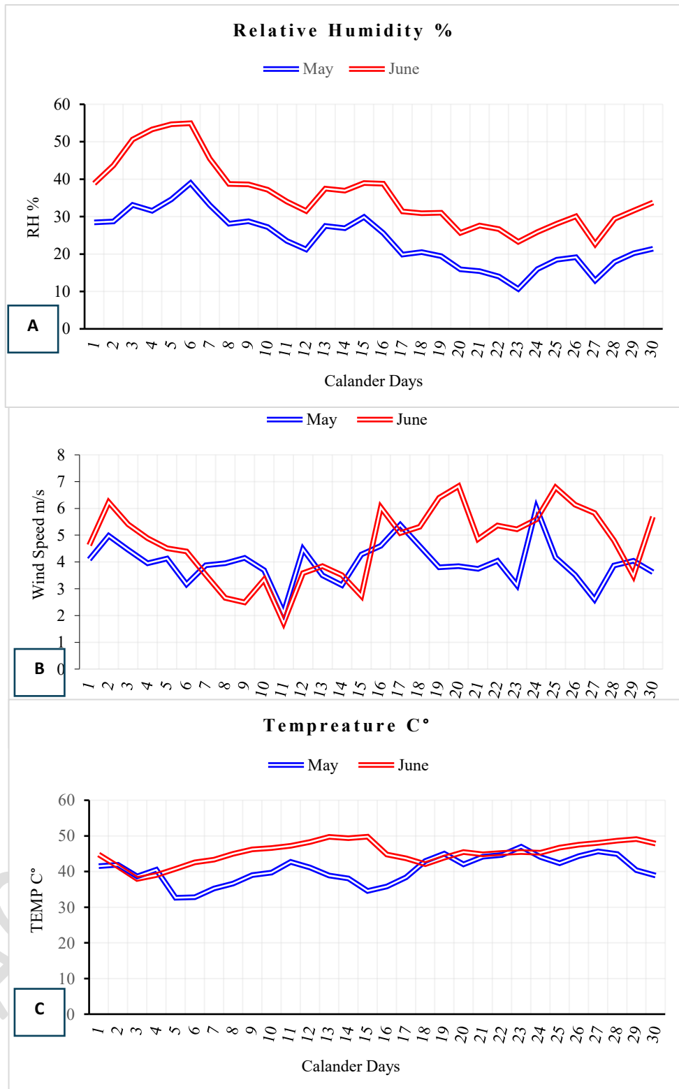
Figure ( 2) Meteorological surface data of the study area during the study period (temperature, wind speed and relative humidity)
