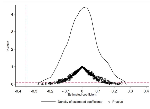
Figure 3. Placebo test.
