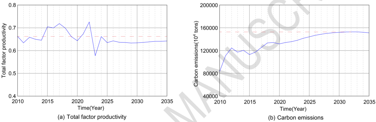
293 294 Fig. 3. Baseline scenario simulation results
