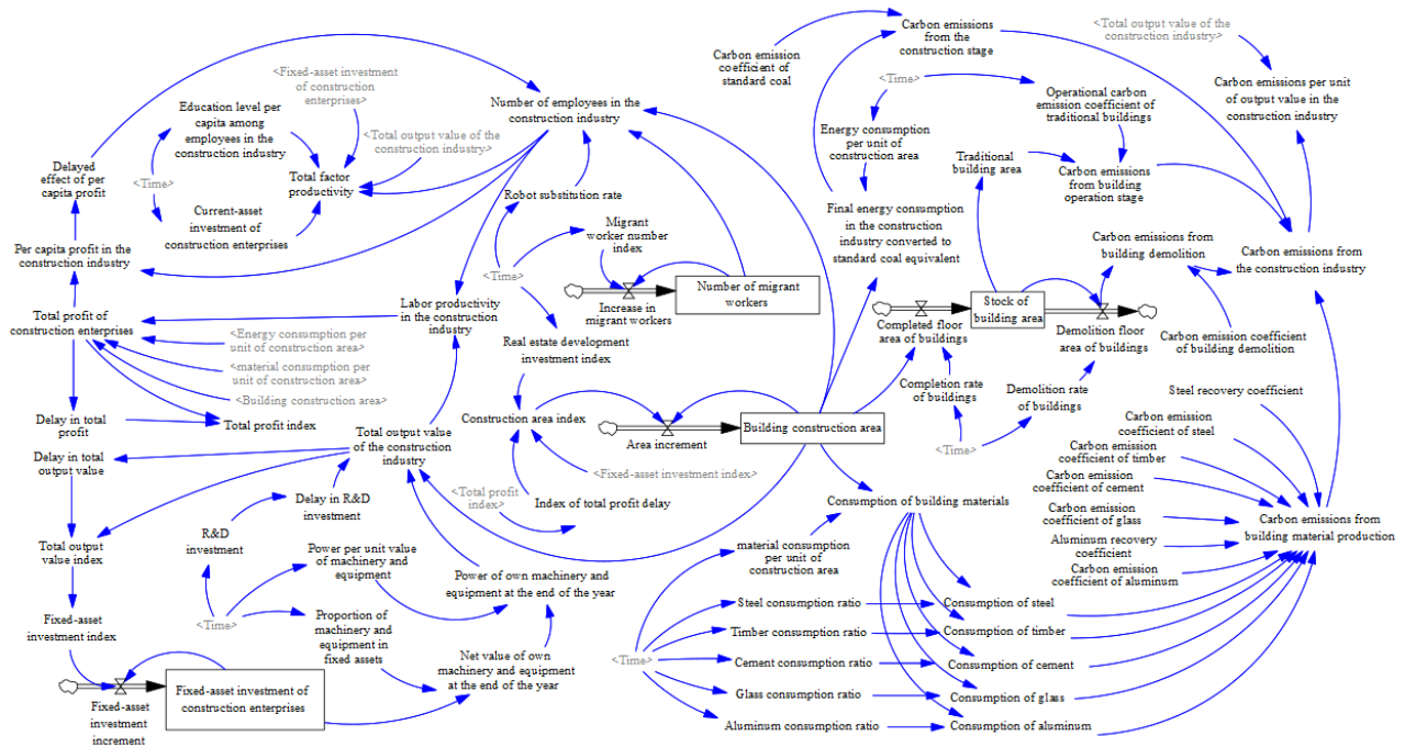
Fig. 2. Stock flow diagram
