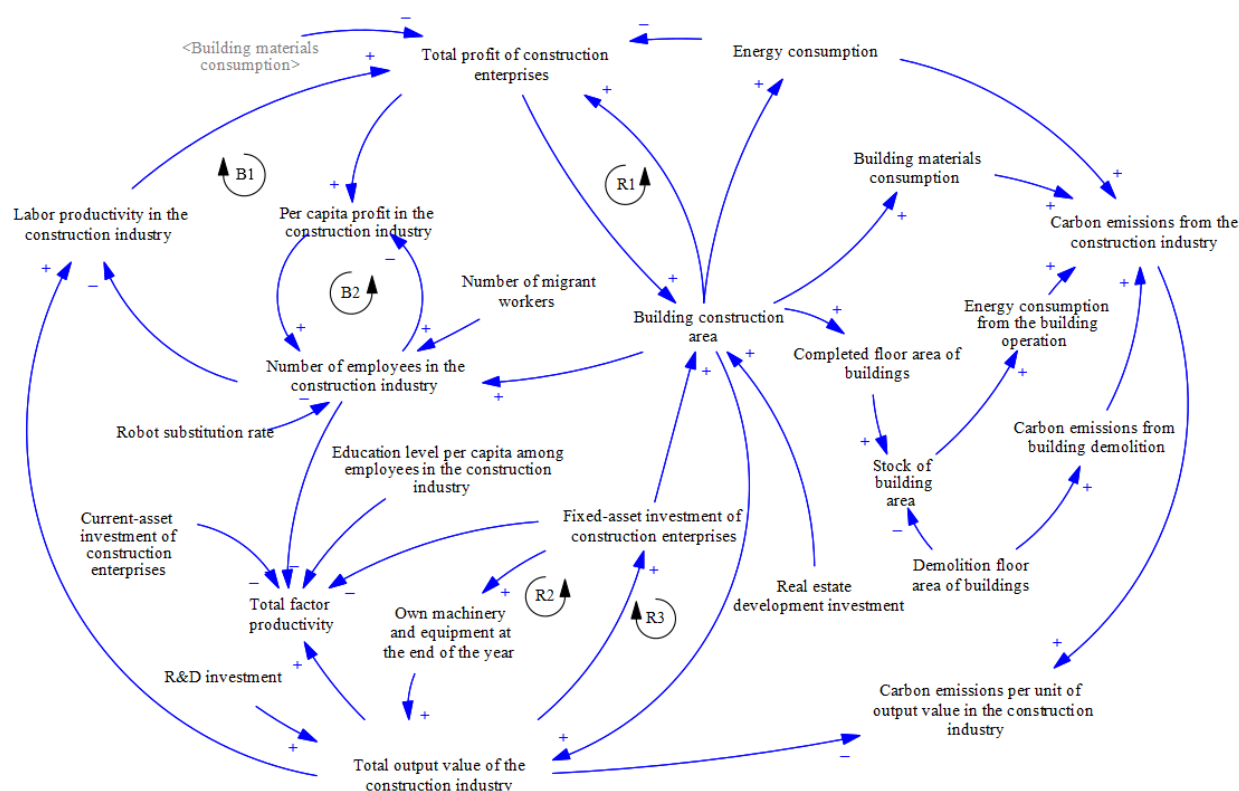
Fig. 1. Causal loop diagram
