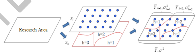
Figure 3. Schematic Diagram of the Working Principle of a Geographic Detector
