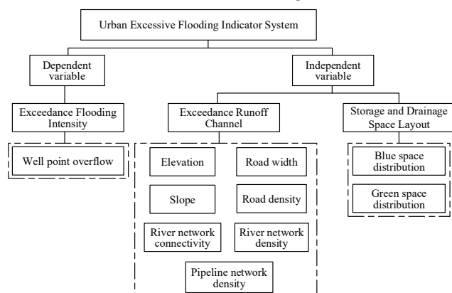
Figure 2. Indicator system
