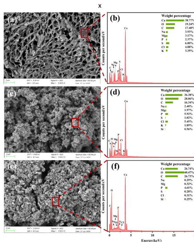
Figure 6. Surface morphology and elemental composition of biochar before and after reaction: (a) and (b) CFS800; (c) and (d) BCFS800; (e) and (f) post-reaction BCFS800.
