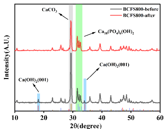
Figure 7. XRD patterns of BCFS800 before and after BPA removal.
