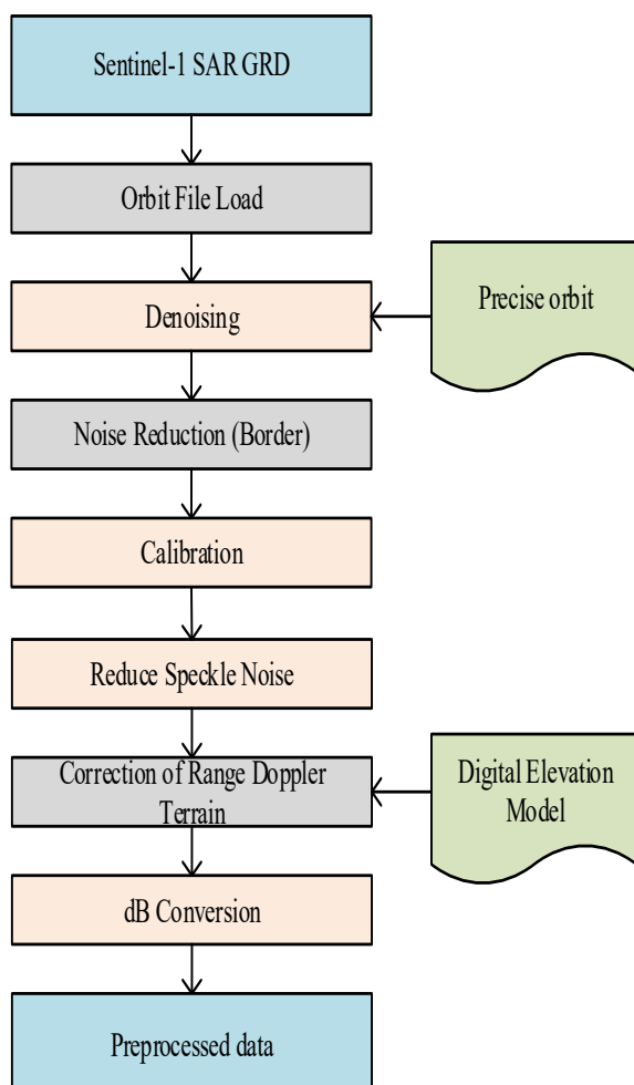
Figure 1. Data Preprocessing Flowchart.
