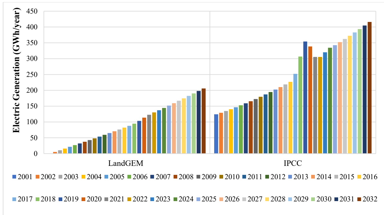
Figure 7. Energy recovery potential from LFG emissions at the Erbil landfill site (2001–2032).
