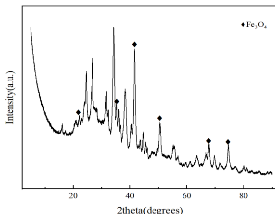
Fig.3 XRD pattern of RM-BC
