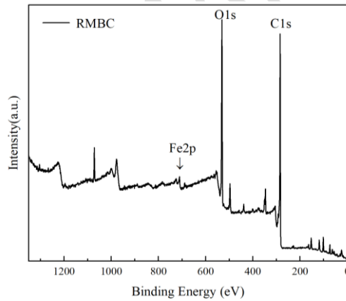
Fig.4 XPS full spectrum of RM-BC
