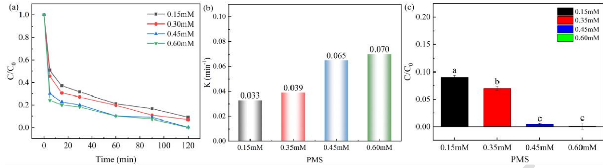
Fig.8 Effect of different PMS dosage on TC removal
