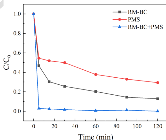
Fig.6 Removal rate of TC under different systems
