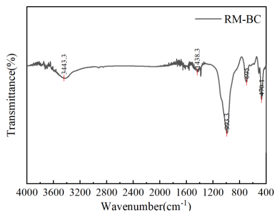
Fig.2 FT-IR spectra of RM-BC
