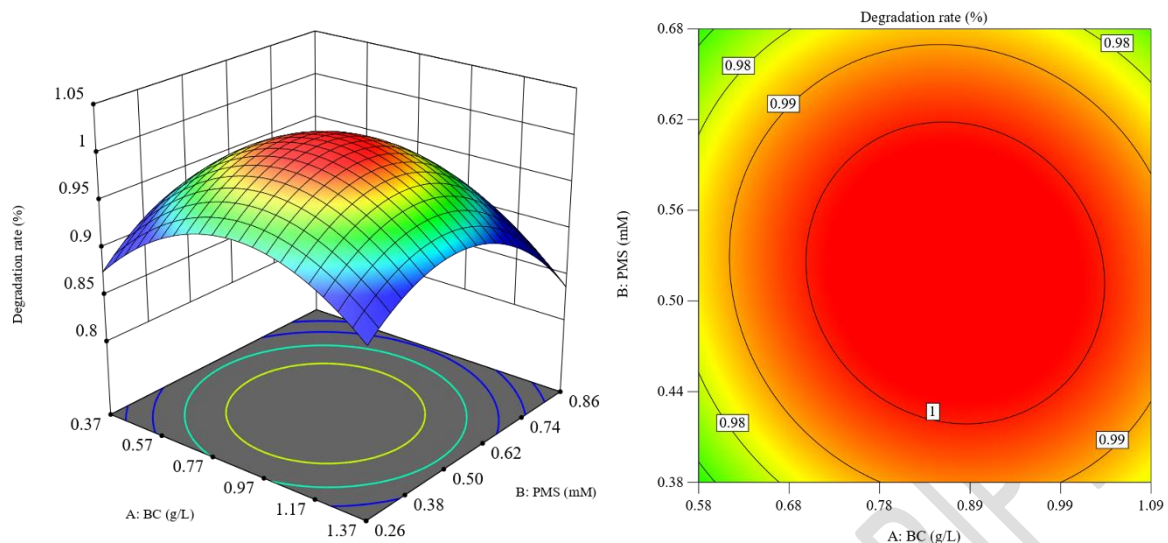
Fig.19 Interaction between biochar dosage and PMS dosage (a) 3D response surface plot; (b) contour plot
