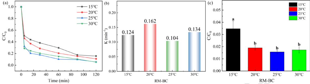
Fig.11 Effect of different reaction temperatures on TC removal
