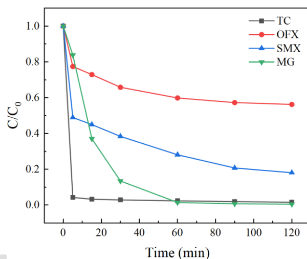
Fig.16 Proficiency testing experiment of RM-BC/PMS reaction system
