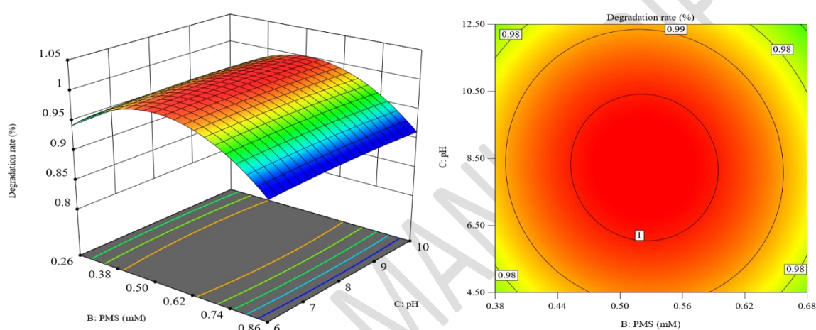
Fig.21 Interaction between the dosage of PMS and the initial pH of the solution (a) 3D response surface plot; (b) contour plot
