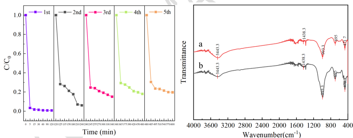
Fig.15 Removal effect of reusing a material of five times, FTIR spectra of the as-prepared catalyst before reaction (a) and after five consecutive reuse cycles (b)
