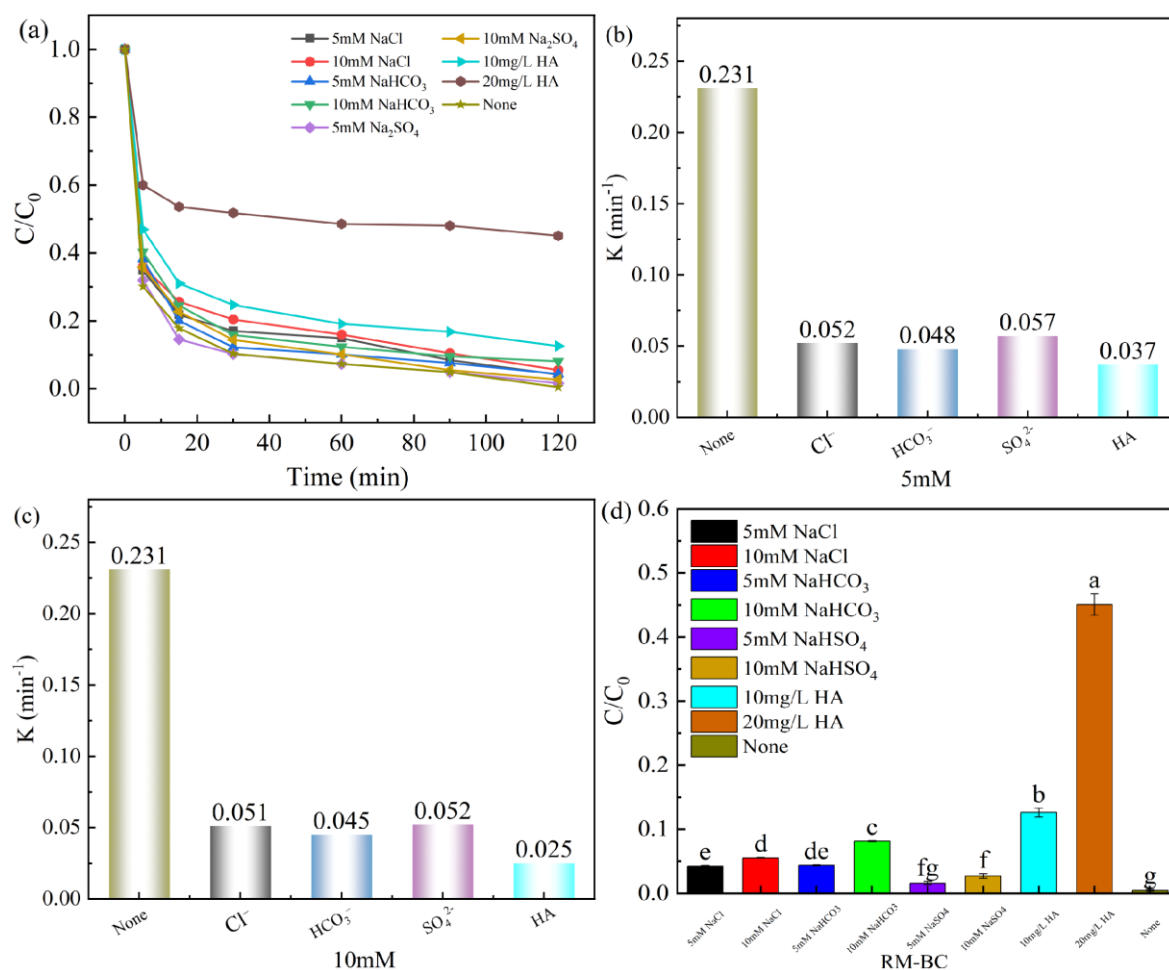
Fig.10 Effect of different interfering ions on TC removal
