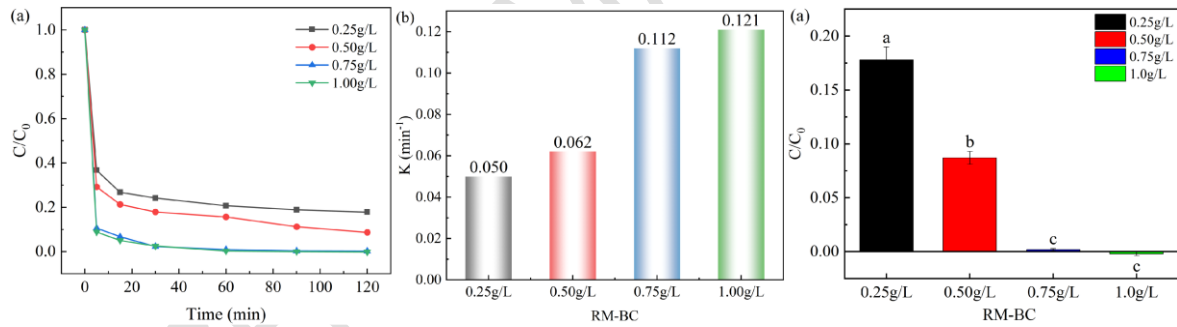
Fig.7 Effect of RM-BC dosage on TC removal
