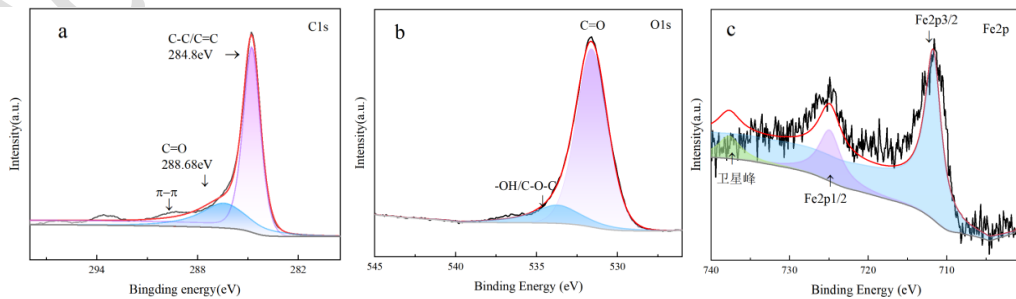
Fig.5 High-resolution XPS spectra of RM-BC: (a) C 1s, (b) O 1s, and (c) Fe 2p.
