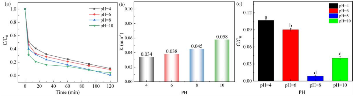
Fig.9 Effect of different pH on TC removal
