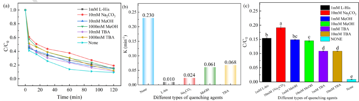
Fig.13 Free radical identification experiments
