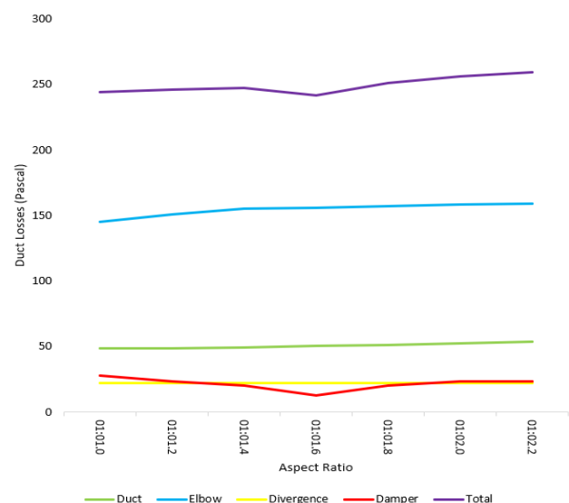
Figure 6 Duct Losses vs Aspect Ratio
