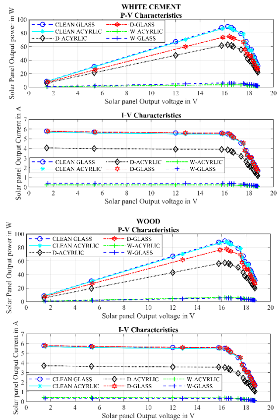
Figure 24 Electrical P-V and I-V Characteristics Curve of Solar Panel under dust samples a) White Cement b) Wood
