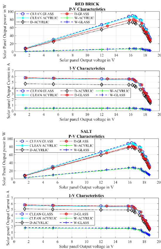
Figure 22 Electrical P-V and I-V Characteristics Curve of Solar Panel under dust samples a) Redbrick b) Salt
