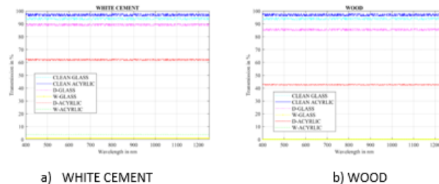
Figure 16 Spectral Transmittance Curve for dust samples a) White Cement b) Wood
