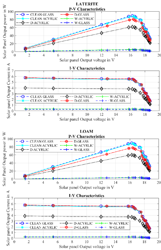
Figure 21 Electrical P-V and I-V Characteristics Curve of Solar Panel under dust samples a) Laterite b) Loamy
