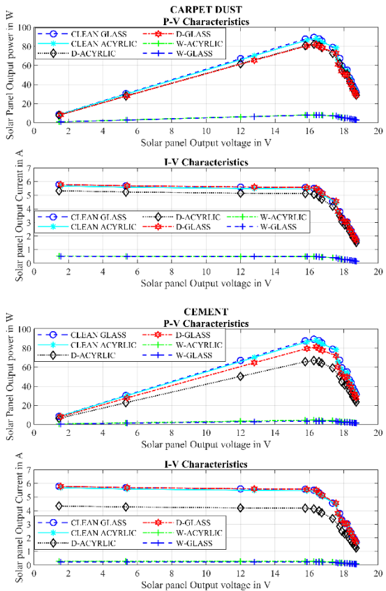
Figure 18 Electrical P-V and I-V Characteristics Curve of Solar Panel under dust samples a) Carpet b) Cement
