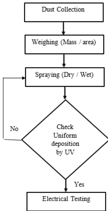
Figure 2(b). Process of Dust Deposition
