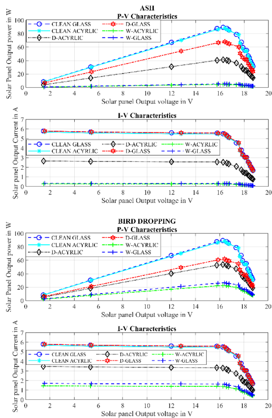
Figure 17 Electrical P-V and I-V Characteristics Curve of Solar Panel under dust samples a) Ash b) Bird dropping
