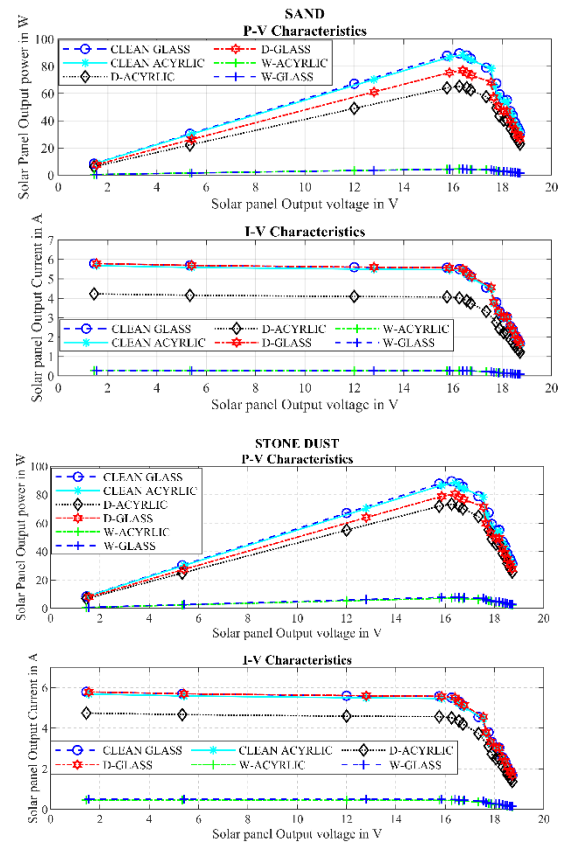
Figure 23 Electrical P-V and I-V Characteristics Curve of Solar Panel under dust samples a) Sandy b) Stone
