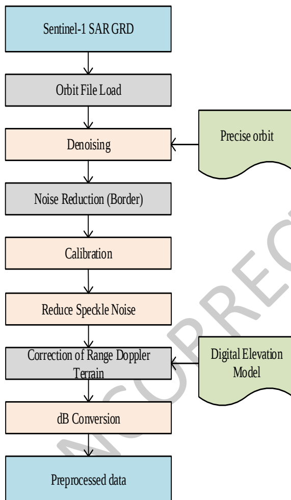
Figure 1. Data Preprocessing Flowchart.
