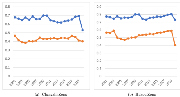
Figure 8. Coupling and coordination degree of Changzhi and Hukou Zones of Shanxi
