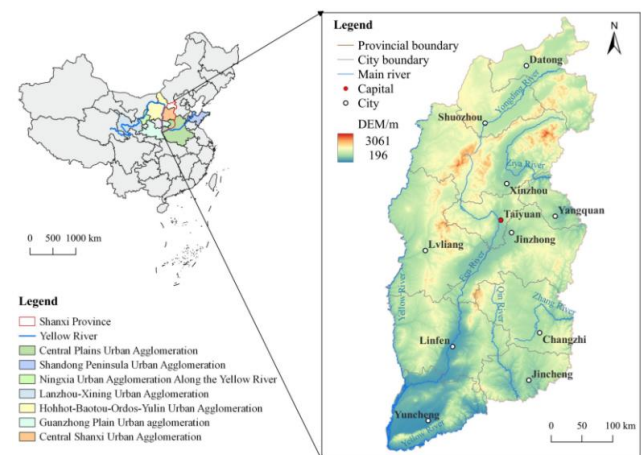
Figure 2. Geographical location of Shanxi province.
