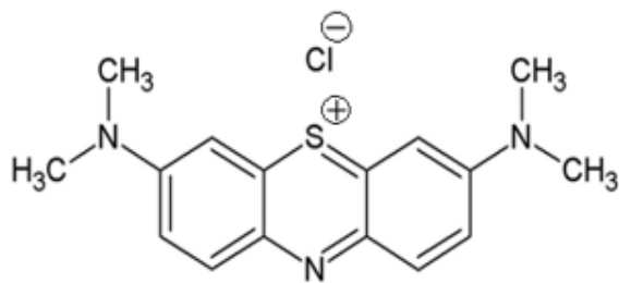
Figure 1. Chemical structure of methylene blue MB
