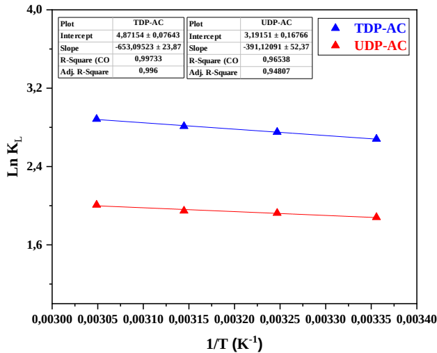
Figure 16. Van't Hoff plots for the adsorption of MB onto UDP-AC and TDP-AC
