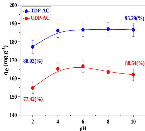
Figure 10. Effect of initial pH on MB adsorption capacity
