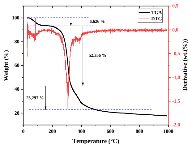
Figure 7. TGA/DTA curves of date pits
