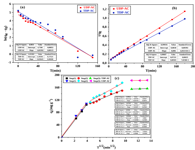
Figure 12. Pseudo-first-order (a), Pseudo-second-order (b) plots and intra-particle diffusion (c) plots of MB adsorption for UDP-AC and TDP-AC
