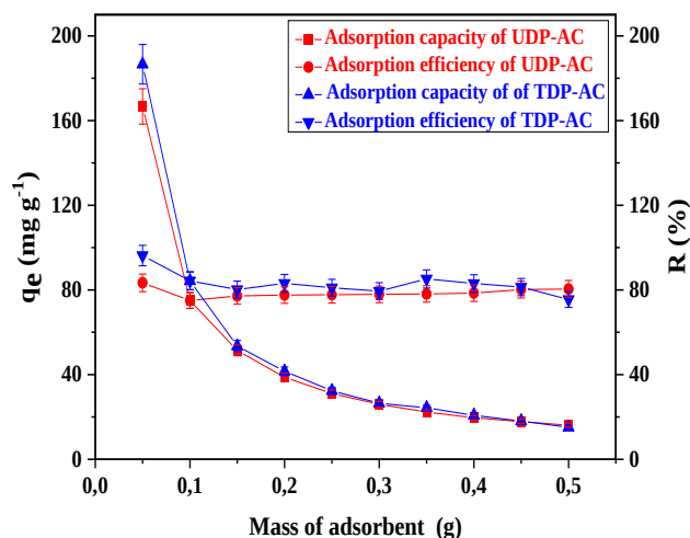
Figure 9. Effect of adsorbent dosage on adsorption of MB by UDP-AC and TDP-AC
