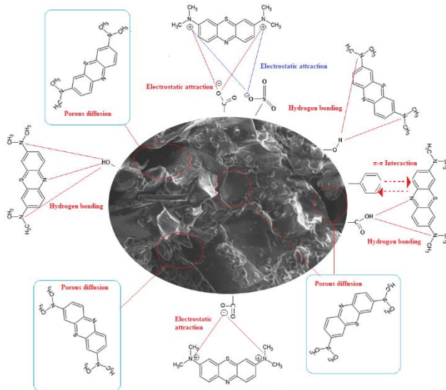
Figure 17. Possible mechanisms for MB adsorption onto TDP-AC
