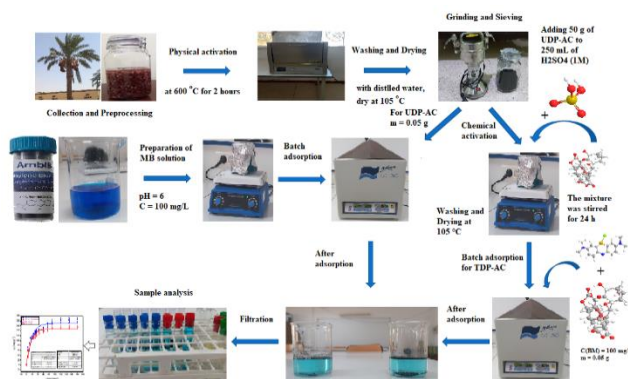
Figure 2. Stages of adsorbent material preparation and Batch adsorption process (C 0 = 100 mg L -1 , pH 6, t = 120 min)
