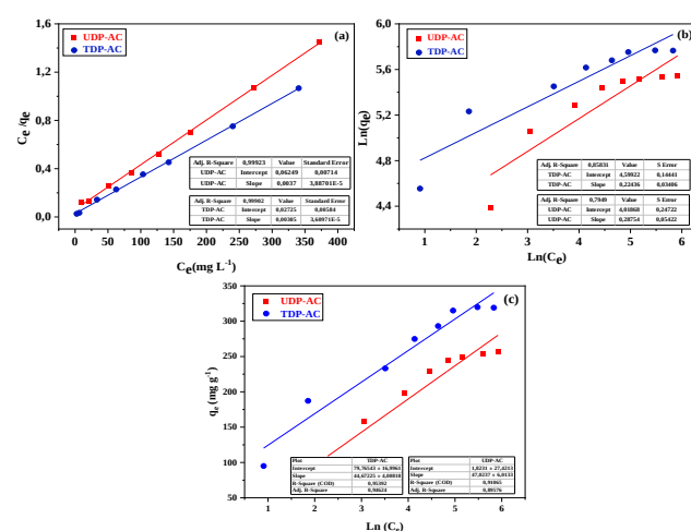
Figure 14. Plot of linear forms of Langmuir (a), Freundlich (b) and Temkin isotherm models for the adsorption of UDP-AC and TDP-AC
