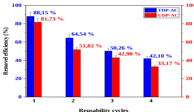
Figure 15. Reusability of TDP-AC and UDP-AC for MB dye
