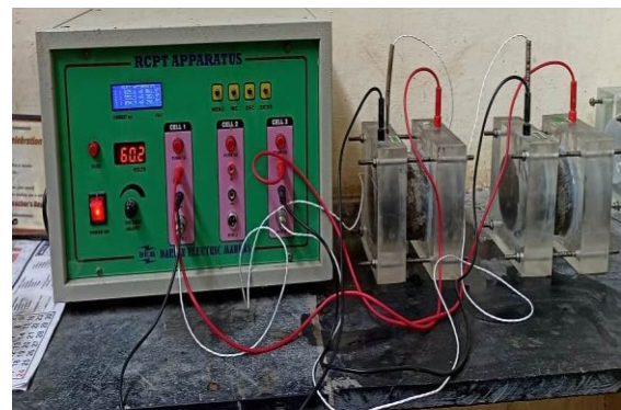
Figure 5. Rapid chloride penetrability test apparatus with specimens
