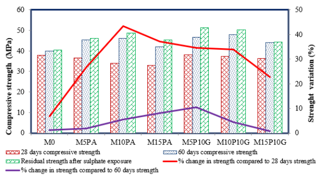
Figure 12. Residual strength observed in the mixtures
