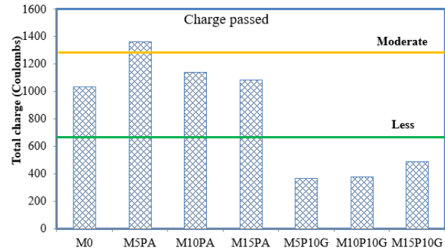
Figure 13. Chloride ion penetrability of concrete composites
