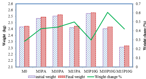
Figure 11. Weight gain of the mixtures with respect to initial weight
