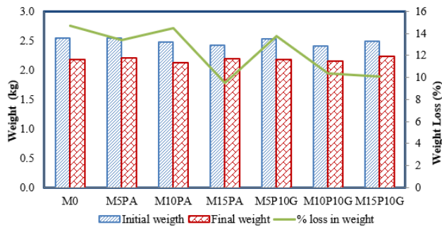
Figure 9. Weight loss observed with respect to initial weight
