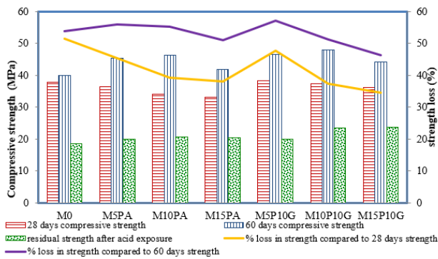
Figure 10. Residual compressive strengths of the mixtures
