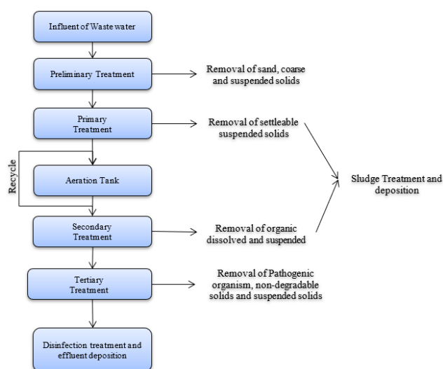
Figure 1. Effluent treatment process
